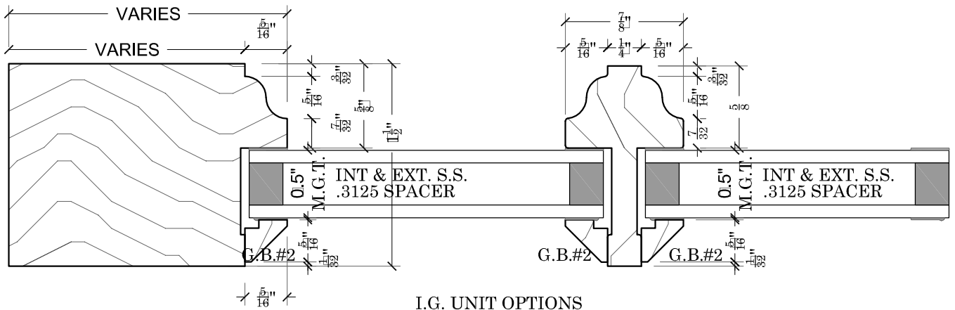
I.G. UNIT OPTIONS OPTIONAL INT OR EXT DOUBLE STRENGTH ANNEALED OR TEMPERED ARGON WITH EXT LOW-E I-89
